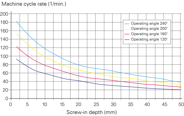
MSE for M5 Phillips screw without torque clutch, p=0.8
