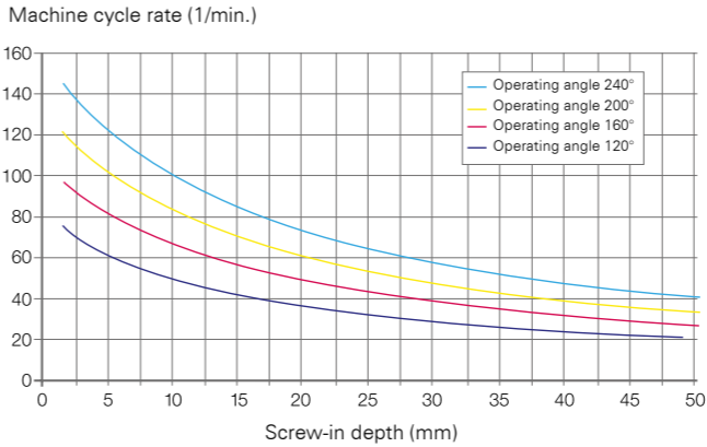
MSE 2 for M5 Phillips screw with torque clutch, p=0.8
